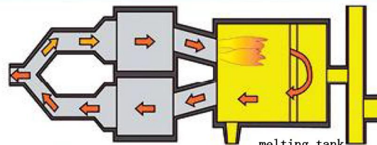
Flue regenerator charging hole material channel
